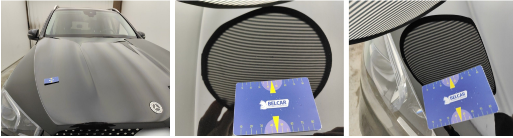
Front Bonnet // Painting-bad repair
