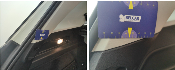
Trunk Compartment / Side Cover Left / Replace-scratch
