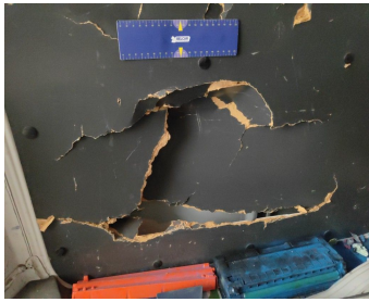
Trunk Lid Interior Coating / MDF Side Door Left / Replace-cracked
